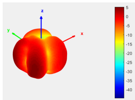
Radiation Pattern at 9GHz
