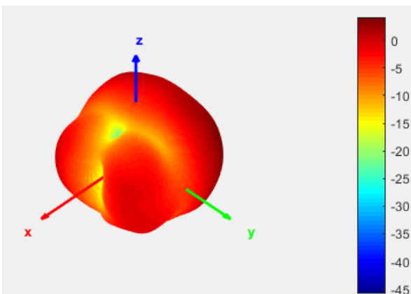
Radiation Pattern at 9GHz
