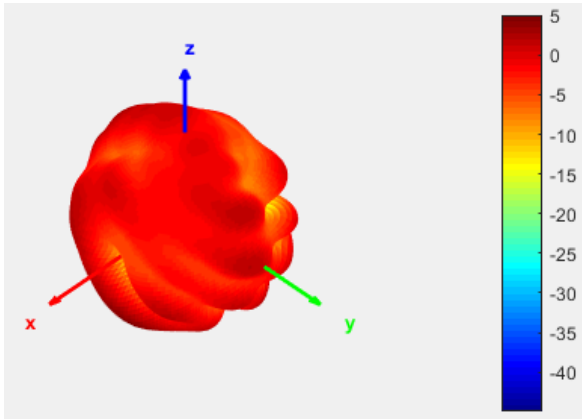
Radiation Pattern at 6.5GHz
