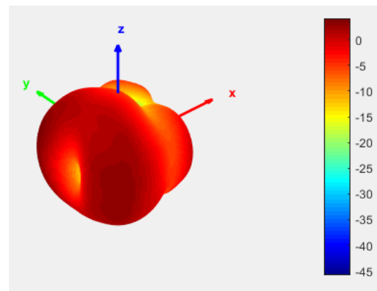
Radiation Pattern at 9GHz
