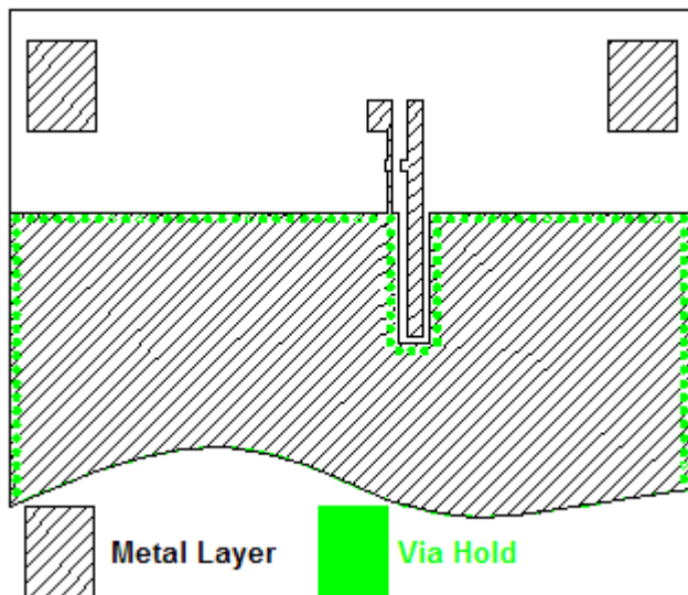
Figure 4. Via holes fence.
