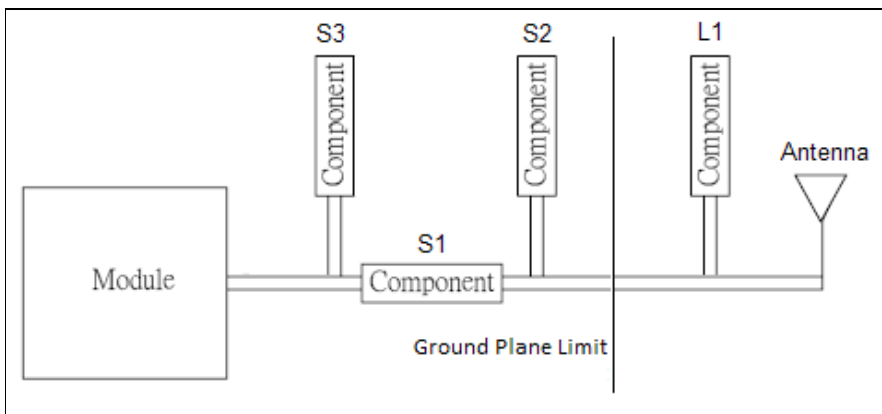
Figure 5. Matching circuit.
