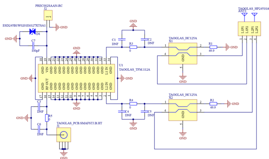
Schematic above shows how the TFM.112A and HP24510A are integrated.
