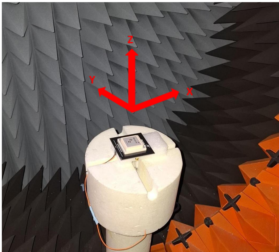
Chamber Test Set-up
