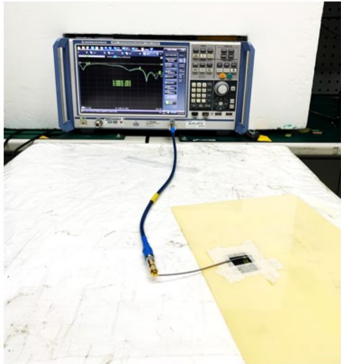
VNA Setup
