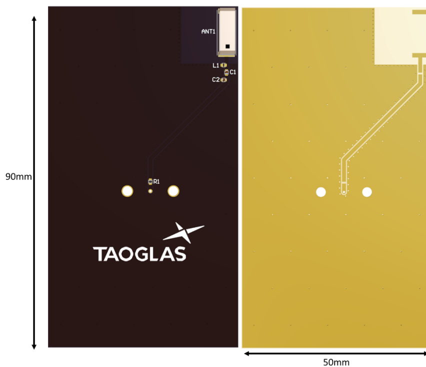
Top Side (ILA.89 placement on 90x50mm PCB reference design)
