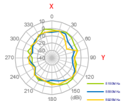
XY Plane
