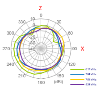
XZ Plane
