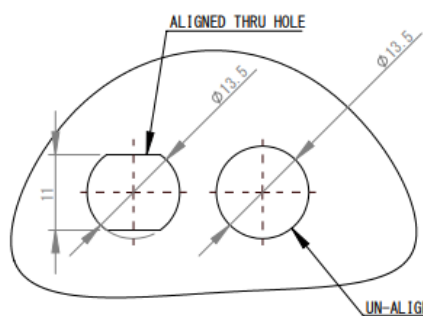
Mounting Hole Recommendation
