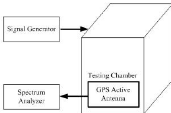
Testing Chamber
