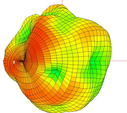
MIMO 2 – 30cmx30cm Ground Plane
