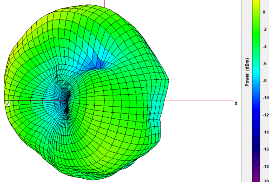
MIMO 1 – 30cmx30cm Ground Plane
