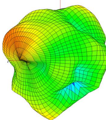
MIMO 2 – Free Space
