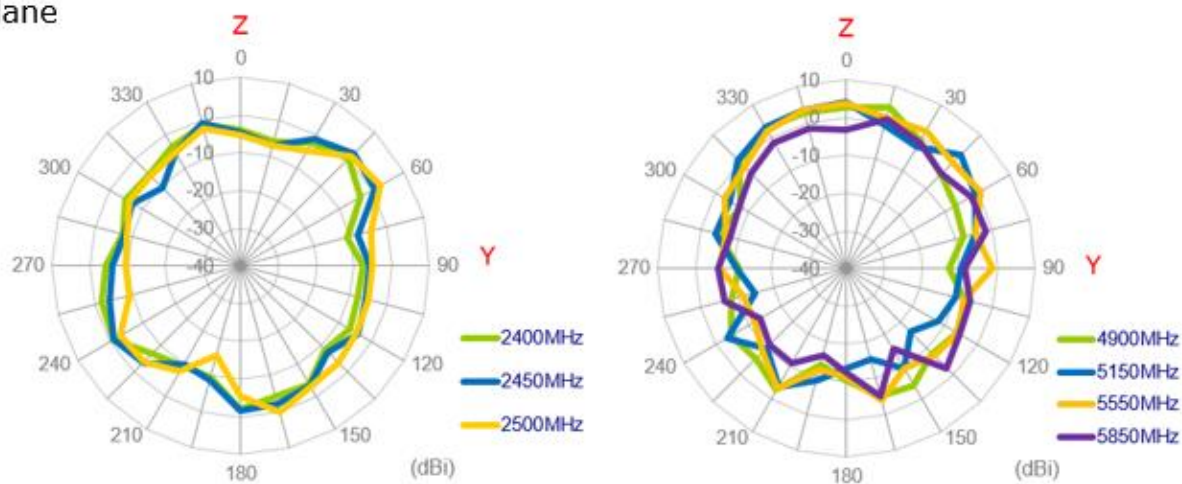
YZ Plane
