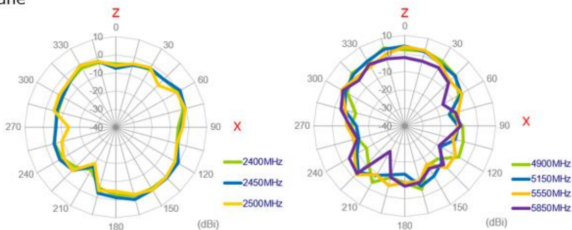
XZ Plane
