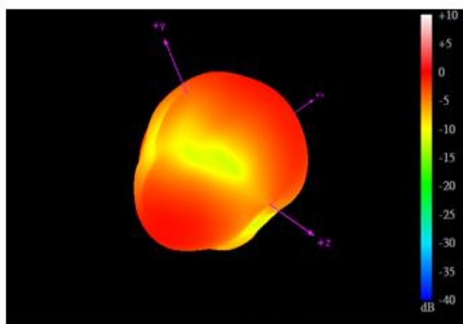
1575.42MHz
