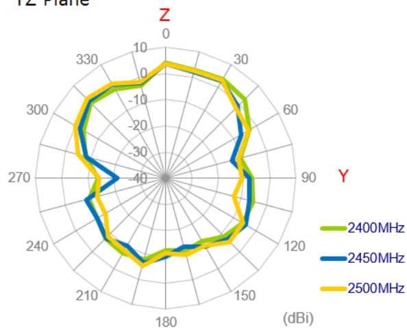
YZ Plane
