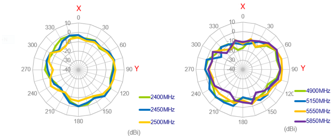
XY Plane
