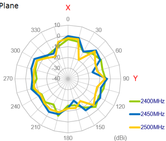
XY Plane
