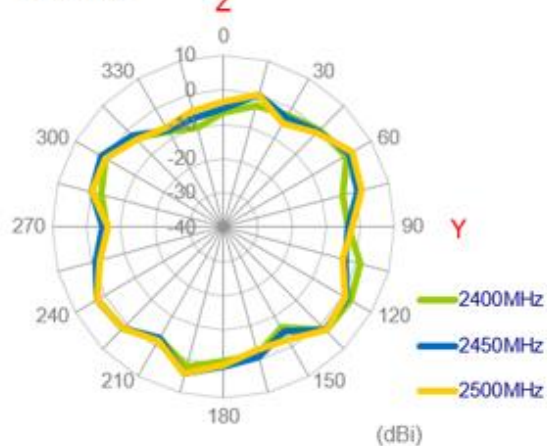
YZ Plane
