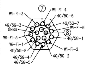
Inside Cable Rubber (Top View)
