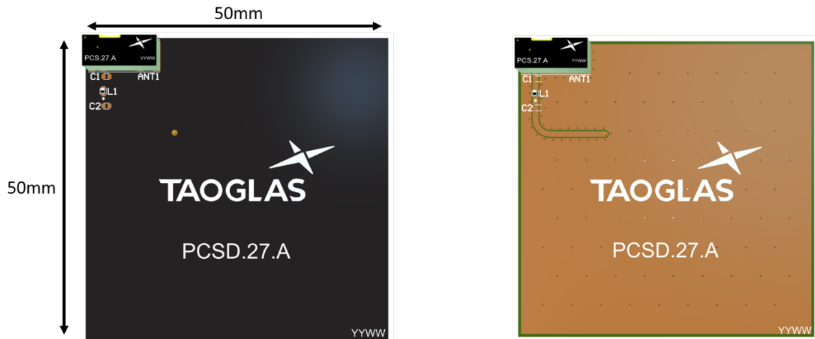
Top Side (PCS.27.A placement on 50x50mm PCB)
