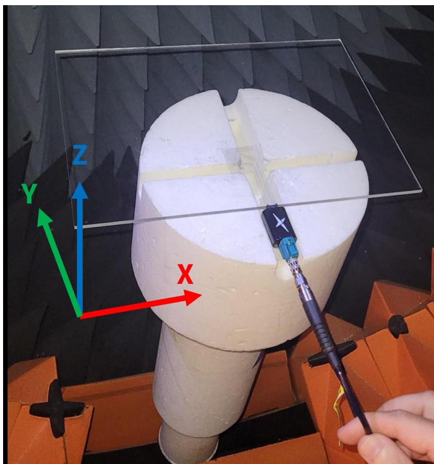
Chamber Test Set-up on 4mm Acrylic
